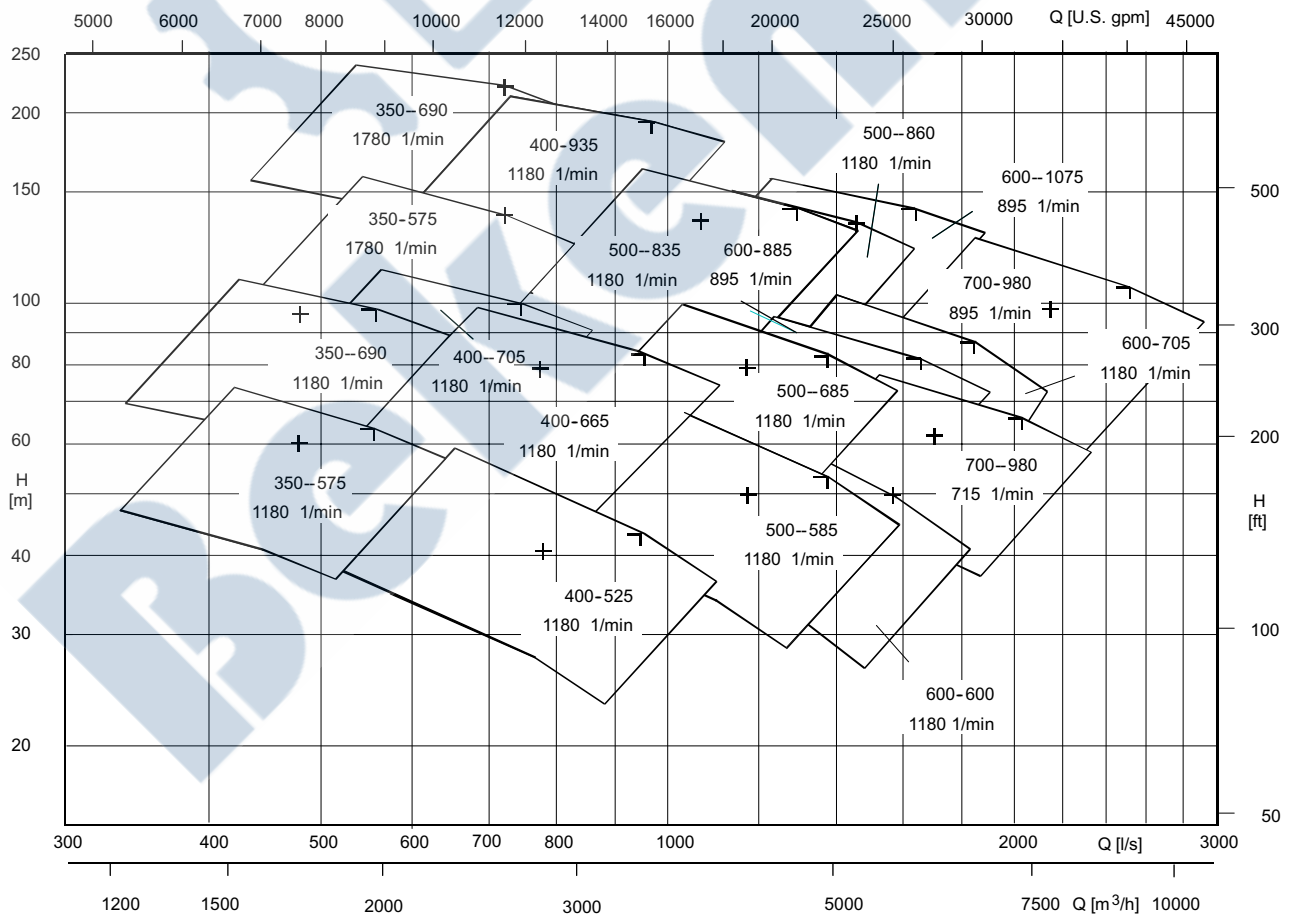
Selection Chart 60 Hz
